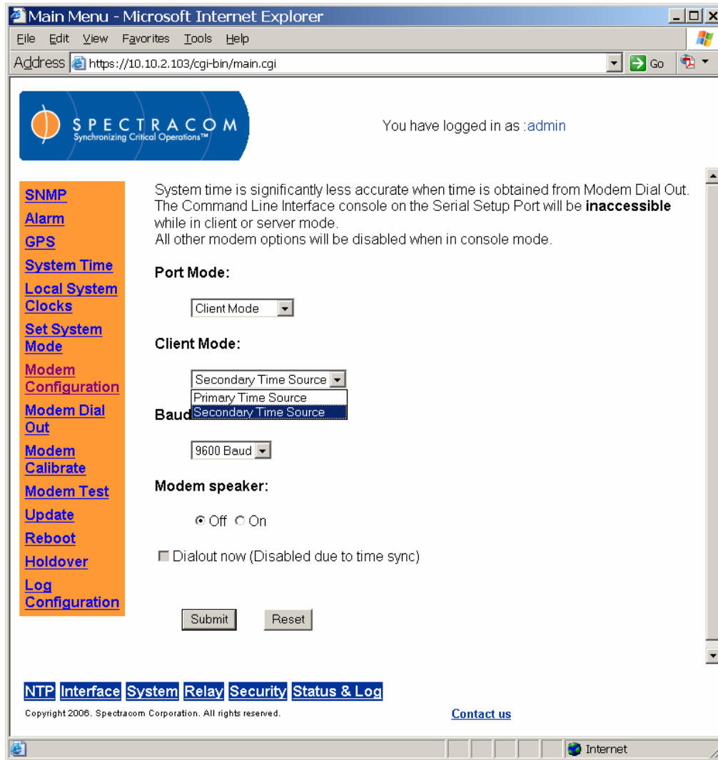
Figure 7-2: System Modem Configuration Screen, Client Mode
