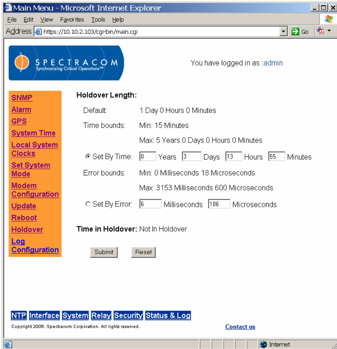
Figure 3-57: System Holdover Screen
