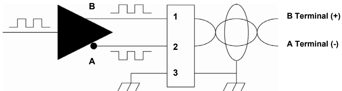
Figure 2-7: RS-485 Output
