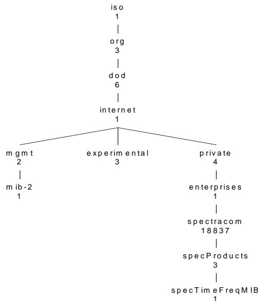
Figure 3-47: Spectracom's MIB
