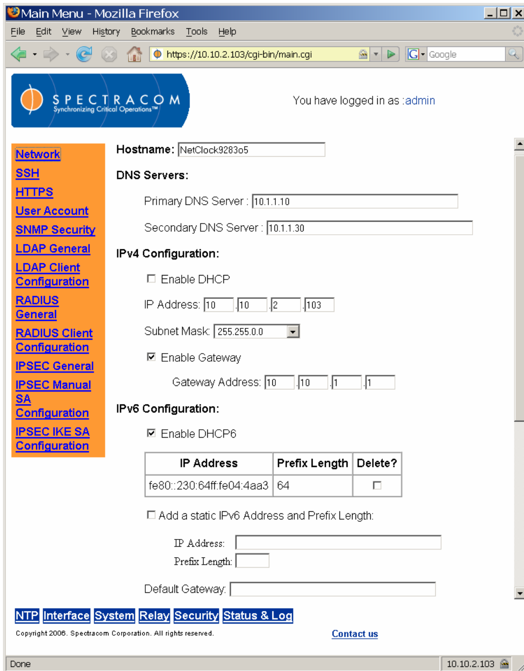
Figure 3-69: Security Network Screen (1 of 2)
