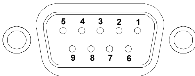
Figure 2-5: Serial Port Pin Configuration
