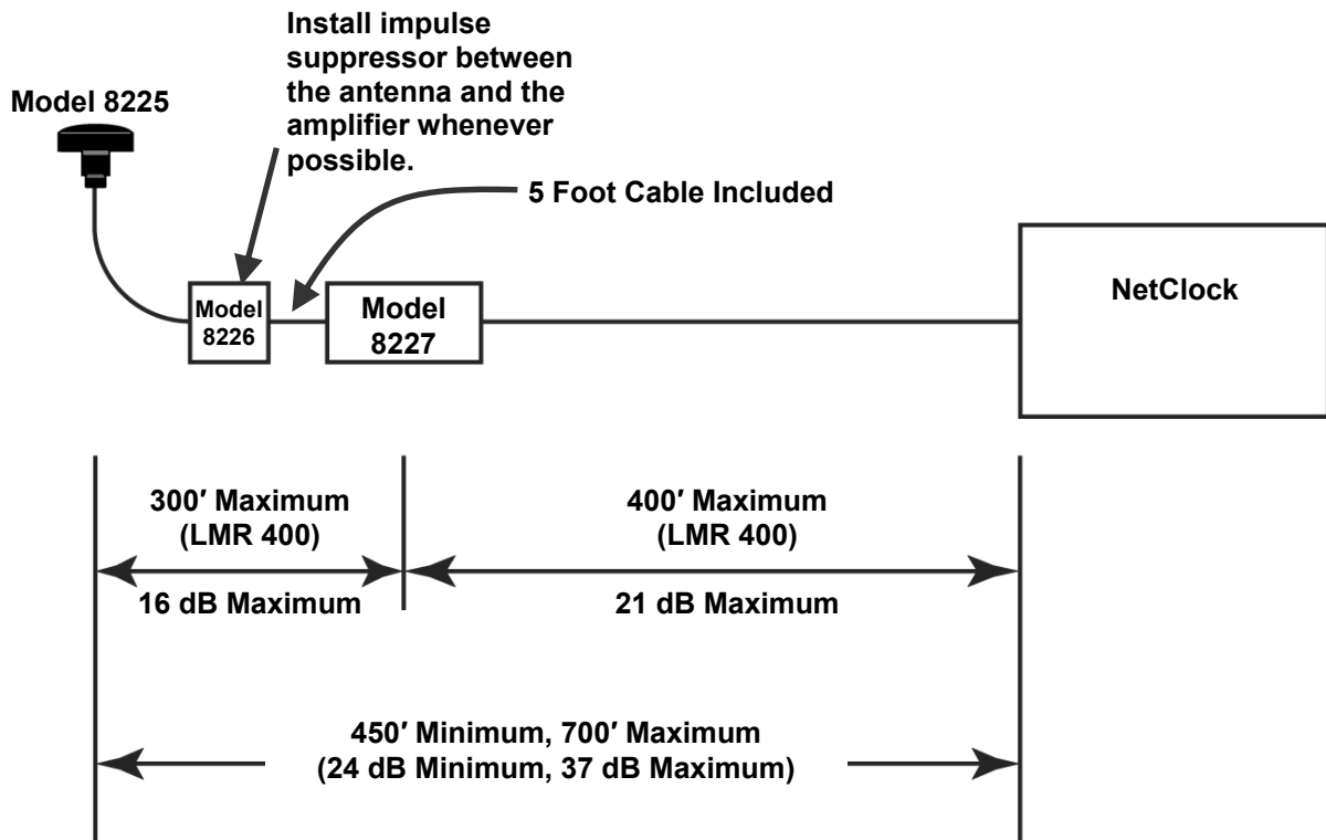
Figure 2-2: Cabling with Inline Amplifier
