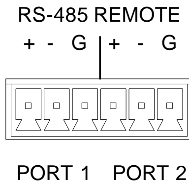
Figure 2-6: Remote Outputs
