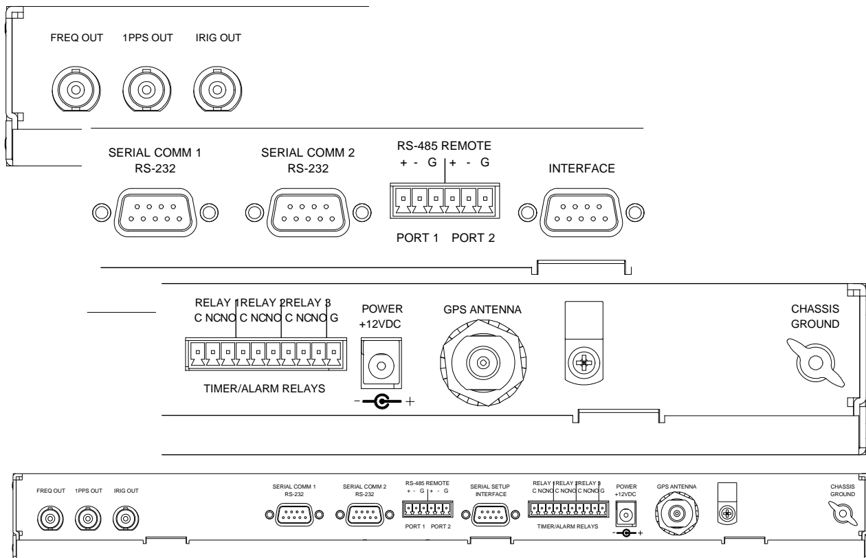
Figure 4-2: NetClock Rear Panel Detail
